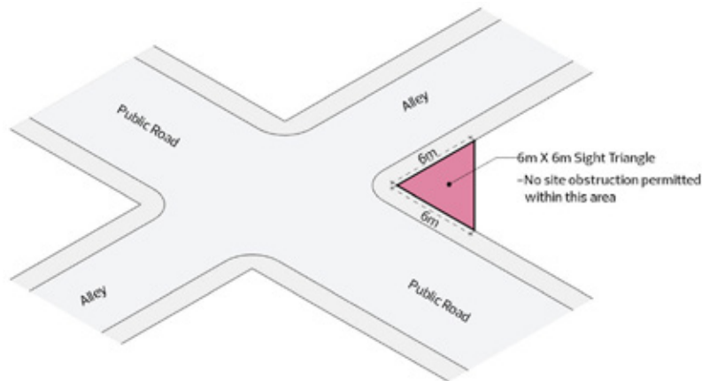
Figure 10 – Sight Triangle
